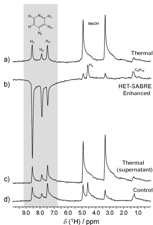
Figure 1. a) Proton NMR spectrum from a degassed mixture containing [\text{D}_4]\text{MeOH} , the HET-SABRE catalyst particles, and the [\text{H}_5]\text{Py} substrate thermally polarized at 9.4 T. b) Corresponding HET-SABRE spectrum obtained from the sample immediately after administration of \text{pH}_2 gas, agitation at about 100 G, and rapid transfer to the 9.4 T NMR magnet. c) Thermally polarized proton NMR spectrum from a supernatant solution. The corresponding control experiment using the supernatant solution is shown in (d) and no SABRE enhancement is observed. All spectra shown were acquired with a single scan ( 90^\circ pulse). Peaks at about \delta = 3.3 and 4.9 ppm are from residual protons from the deuterated solvent. The peak at \delta = 4.5 ppm in (b) and (d) is from \text{H}_2 gas. The peak at \delta = 1.3 is assigned to cyclooctane ( \text{C}_8\text{H}_{16} ). [7g] Spectra from an additional supernatant control experiment, as well as additional experimental details, are provided in the Supporting Information.
