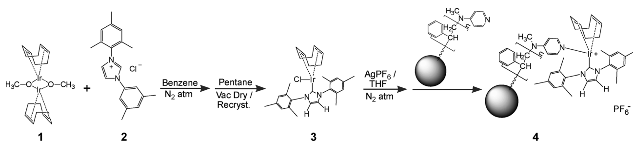
Scheme 1. Relevant structures and a synthetic summary for preparation of the HET-SABRE catalyst studied herein. a) Preparation of the [\text{IrCl}(\text{cod})(\text{IMes})] SABRE catalyst ( 3 ), which is a precursor for the preparation of the covalently linked SABRE catalyst 4 .
